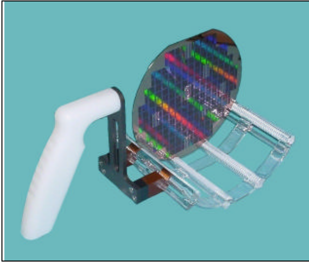
Lever Style with 30° Grip for Quartz Boat
